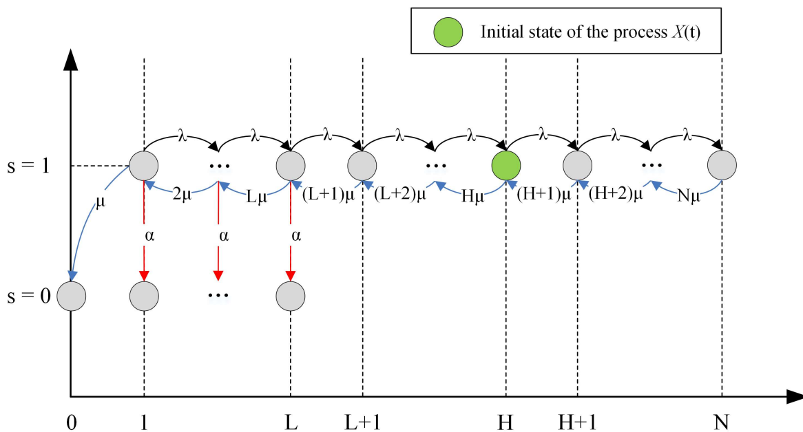
Figure 6. The state transition diagram of the truncated Markov process \hat{\mathcal{X}}(t)
