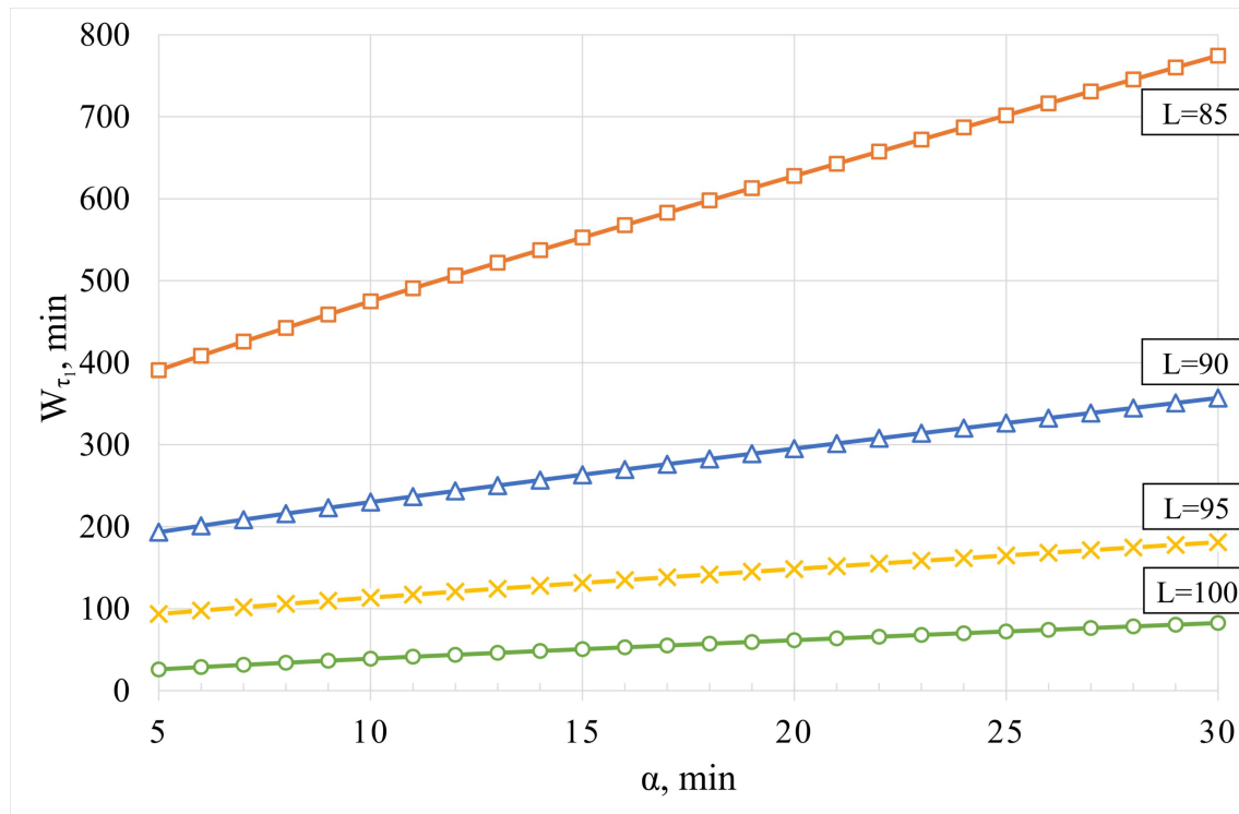
Figure 9. MEC server runtime against the MEC server disabling time for different L
